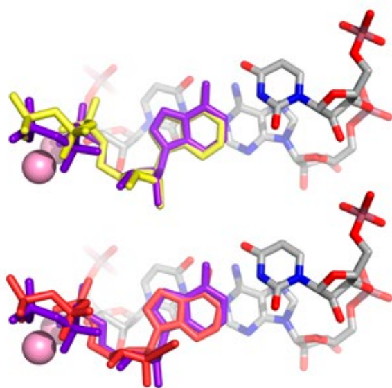
The structural model of Zika virus RNA-dependent RNA polymerase in complex with RNA for the rational design of novel nucleotide inhibitors
