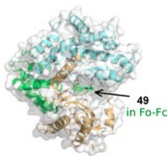
PI4KB kinase crystallize with an inhibitor. (Mejdrova et al. J. Med. Chem. 2015 and 2017)
