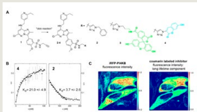
(Left) Design of novel PI4KII \beta inhibitors that are hybrids of MI14 and PIK93. (Up) A) Fluorescent inhibitors as chemical biology tools. B) Biochemical evaluation of fluorescent compound 4 and nonfluorescent analogue 2. C) Colocalization of fluorescent inhibitor 4 with transiently expressed iRFP-PI4KII \beta in living HeLa cells.
